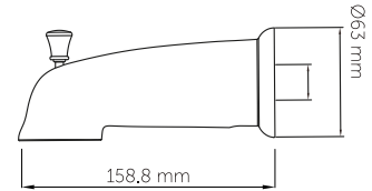
VISTA LATERAL / LATERAL VIEW
