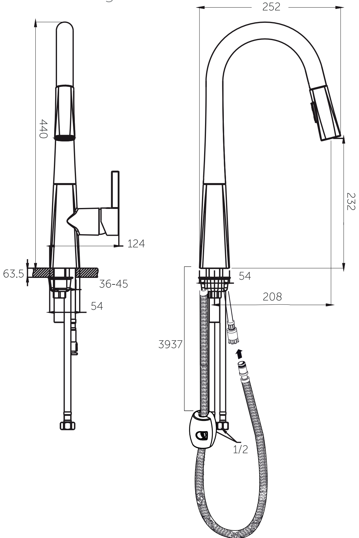
VISTA FRONTAL / FRONT VIEW
